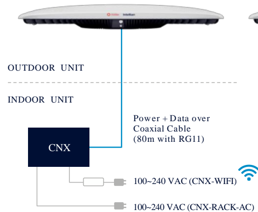
Single Antenna Configuration with CNX
