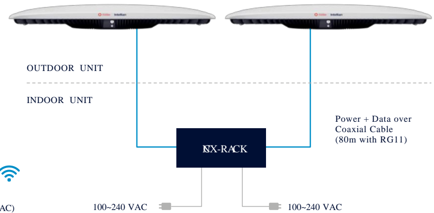
Dual Antenna Configuration with CNX-RACK
